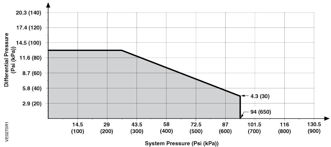
Figure 3. Allowable Differential Pressure in Relation to System Pressure.
