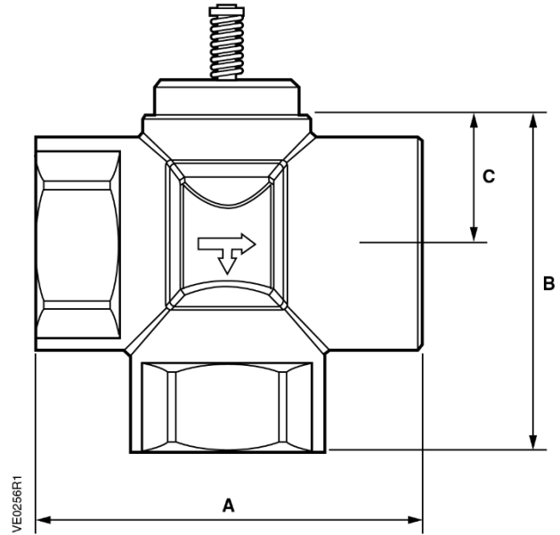
Figure 5. 3-Way Valve Body.
