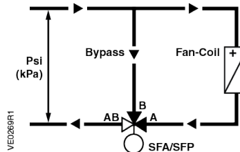
Figure 5. Mounting in the Return Flow.
