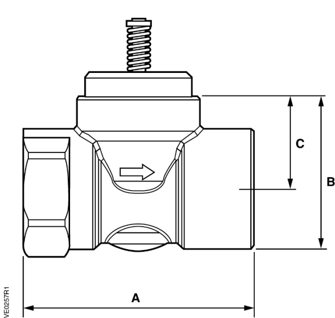
Figure 4. 2-Way Valve Body.
