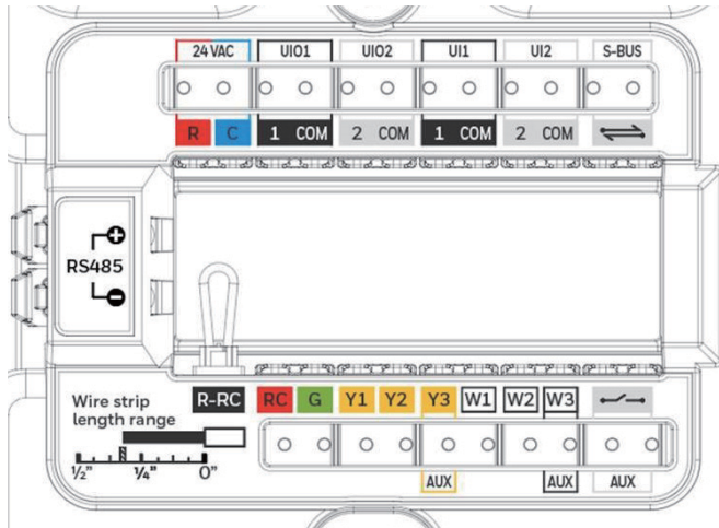
Fig. 1. Terminals
